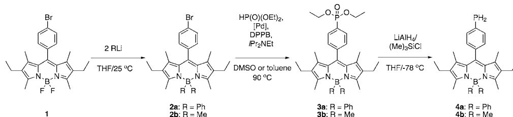
Scheme 1. Synthetic procedure for the novel compounds 2a/2b , 3a/3b , and 4a/b . DPPB = 1,4-bis(diphenylphosphino)butane, DMSO = dimethyl sulfoxide.
